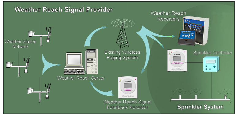
The Weather Reach Water Management System
