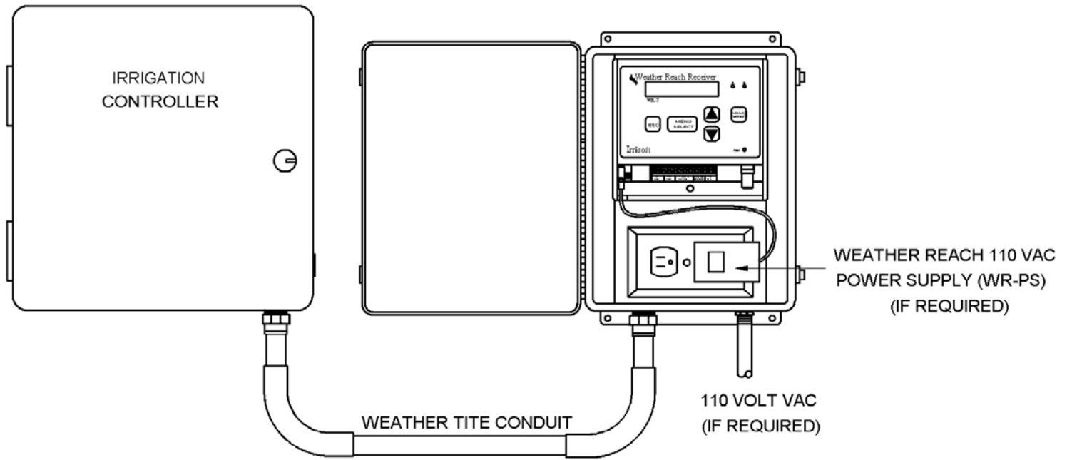
WEATHER REACH RECEIVER (WR-7) INSTALLED IN A WEATHER REACH OUTDOOR ENCLOSURE (WR-0E)
